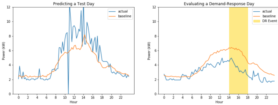
Fig. 20. The left plot displays the prediction of energy consumption in an office building on a test day. The right plot displays a DR event which produced desired results when compared to the baseline—an estimated $10 of savings and 7 kWh reduced energy consumption during the event.
