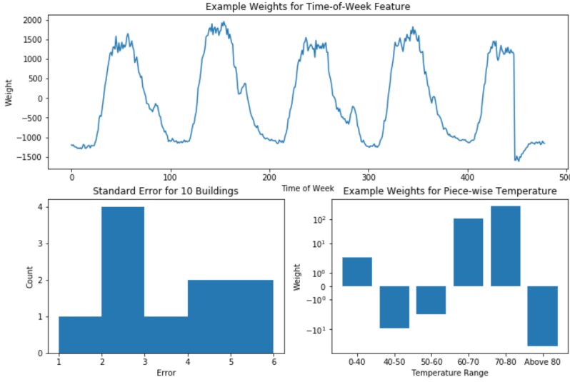
Fig. 21. The bottom-left histogram displays the test standard errors for each of the ten buildings. The top and bottom-right plots display example weights for a baseline model trained for an office building. The model captures the daily period of demand, as well as the non-linear relationship between temperature and demand described in [25]. The weight for temperature change was -39.8.
