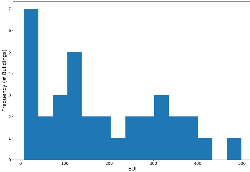
Fig. 10. Distribution of EUI across the Mortar portfolio
