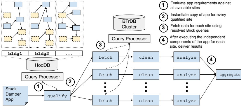
Fig. 4. Architecture of a portable analytics application. An application consists of five segments: qualify which filters the building corpus into the execution set, fetch, clean and analyze which are all executed once for each building in the execution set, and aggregate which is executed once over all outputs of analyze.
