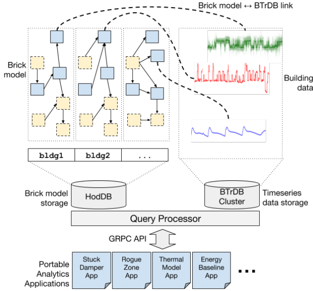
Fig. 1. Mortar architecture
