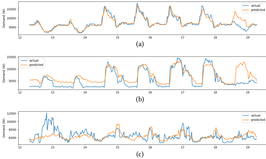
Fig. 12. Baseline prediction app: Predicted baseline using [25] plotted against actual building energy consumption.
