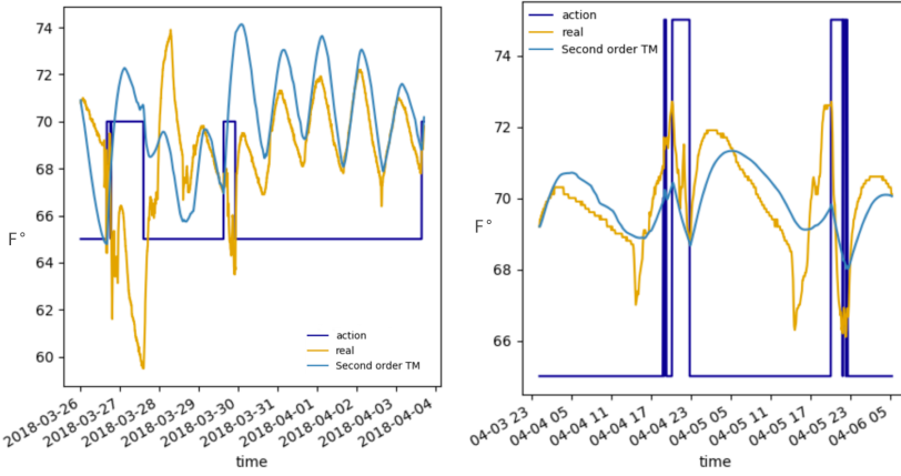
Fig. 22. Forecasting results for a sample site. The “real” line is the true indoor temperature. “Second order TM” line are the forecasting results. The “action” line indicates for the left (right) image whether or not heating (cooling) happened in the given zone.
